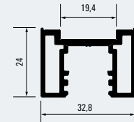
Griffprofil 19 Handle profile 19 100008732
