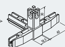
Eckknoten 4 S H Corner joint, 4-sided, horizontal 100003061
