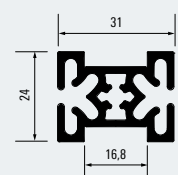
Sprossenprofil 16 Glazing bar profile 16 100008689
