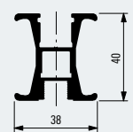
Griffprofil 40 C Handle profile 40 C 100008319
