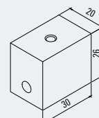
Eckverbinder Türprofil Premium L-XL unten Bottom corner cleat, premium door profile L-XL 100022472
