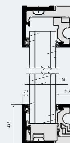
Vertikalschnitt Komplettsystem Isolierglas Vertical section detail of the complete system with insulating glass
