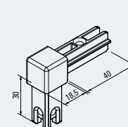
Eckknoten 2 S Corner joint, 2-sided 100003039
