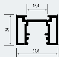
Griffprofil 16 Handle profile 16 100008660
