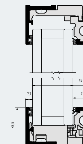
Vertikalschnitt Komplettsystem Schallschutz-Isolierglas Vertical section detail of the complete system with sound reduction insulating glass
