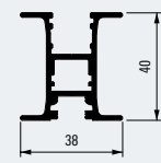
Griffprofil 40 C Basic+ Handle profile 40 C Basic+ 100008359
