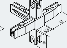
Eckknoten 5 S Corner joint, 5-sided 100003066
