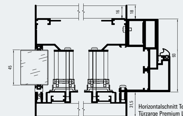
Horizontalschnitt Technikpaneel Türzarge Premium S Horizontal section detail for technical panel for premium door frame trim S
