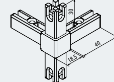
Eckknoten 4 S Corner joint, 4-sided 100003055
