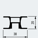
Griffprofil 20 C Handle profile 20 C 100008444
