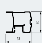
Griffprofil 30 C BAL Bürste Handle profile 30 C BAL brush 100022634
