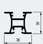
Griffprofil 30 C Handle profile 30 C 100022632
