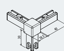
Eckknoten 3 S Corner joint, 3-sided 100003049
