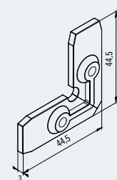
Eckverbinder Türprofil Premium L-XL Corner cleat, premium door profile L-XL 100011927
